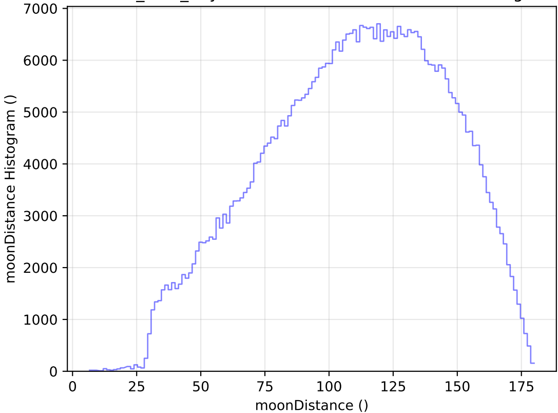
baseline_v3.0_10yrs WFD r band: moonDistance Histogram
