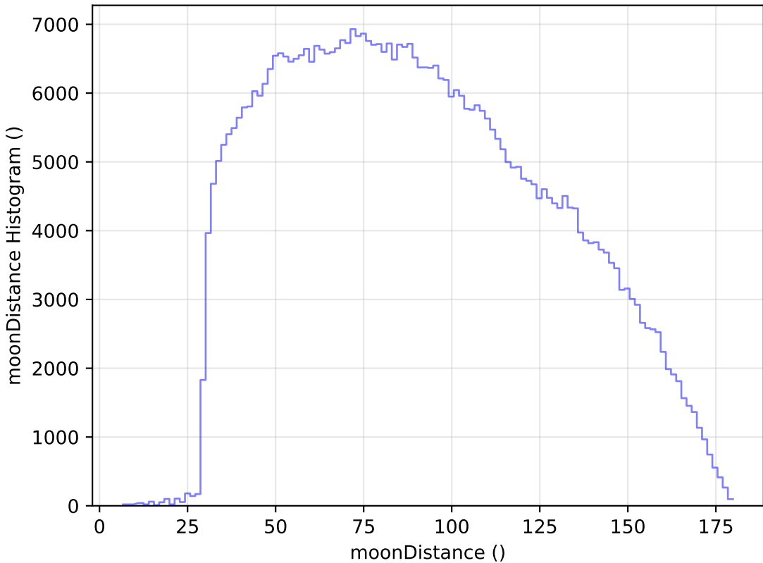
baseline_v3.0_10yrs WFD i band: moonDistance Histogram
