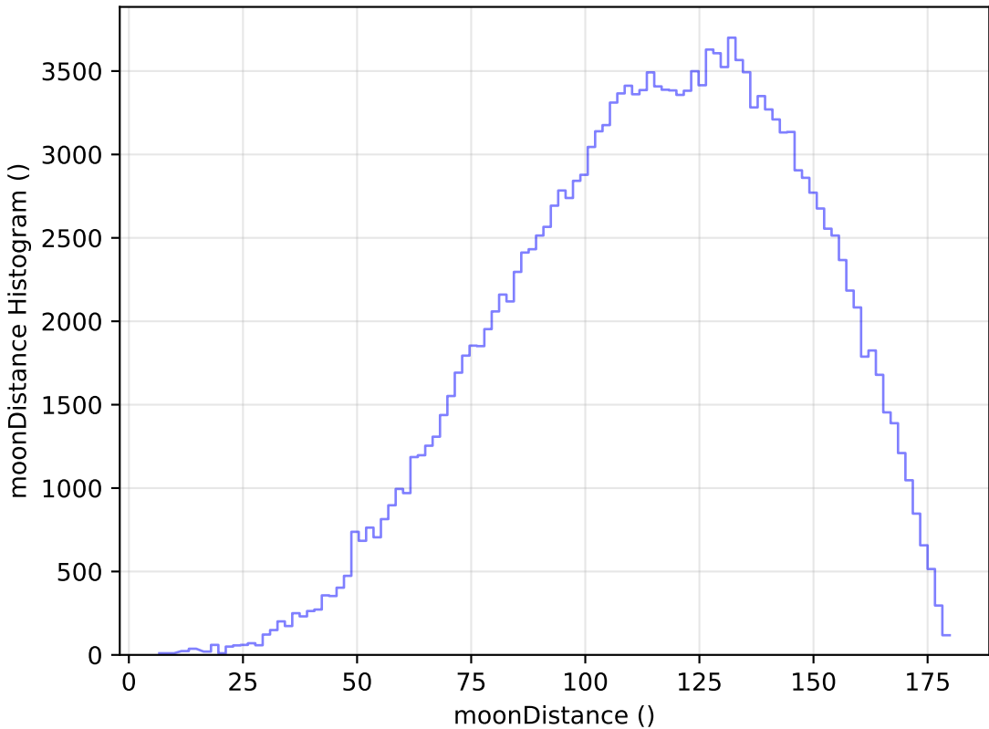
baseline_v3.0_10yrs WFD g band: moonDistance Histogram
