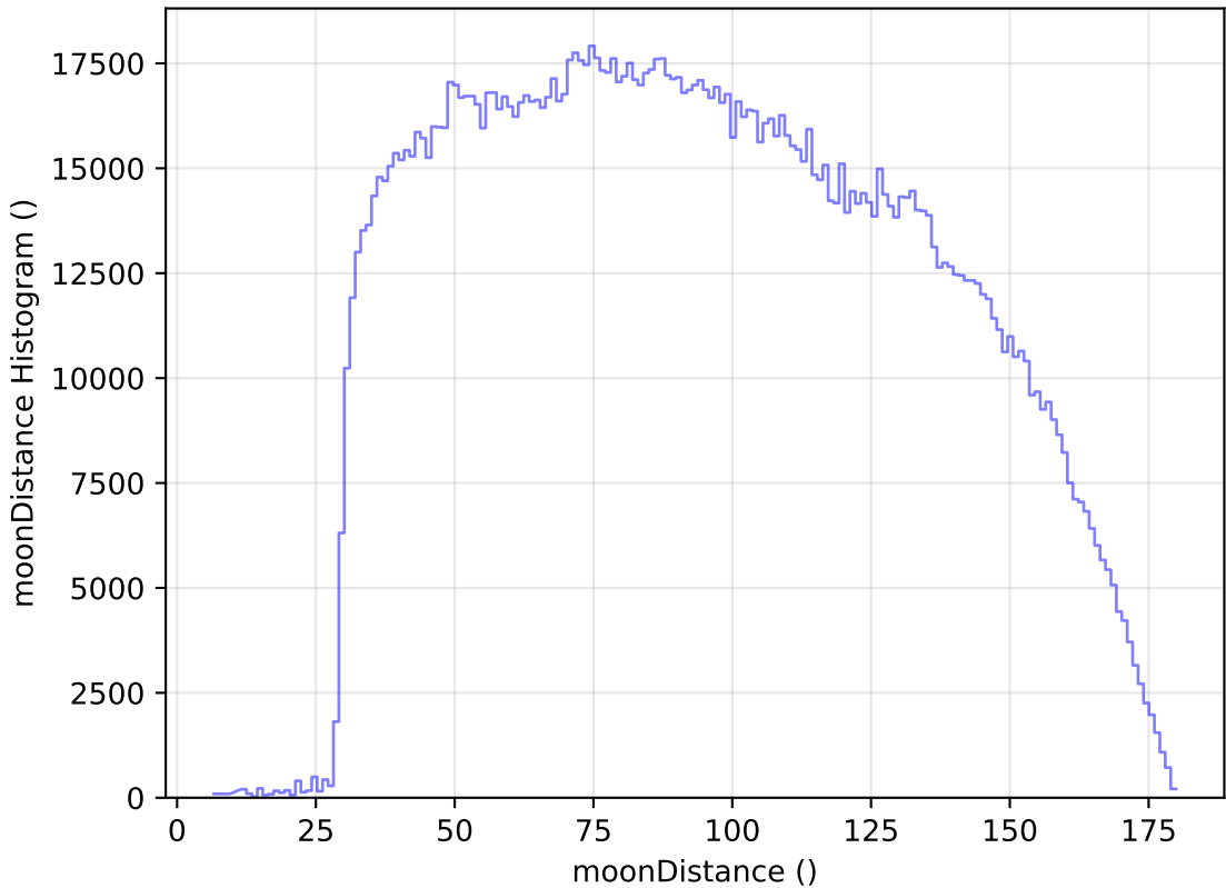
baseline_v3.0_10yrs WFD all bands: moonDistance Histogram
