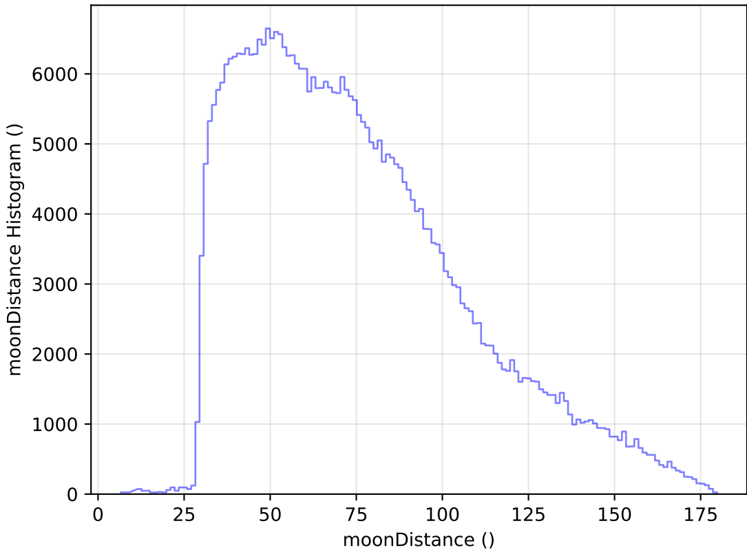
baseline_v3.0_10yrs All sky z band: moonDistance Histogram
