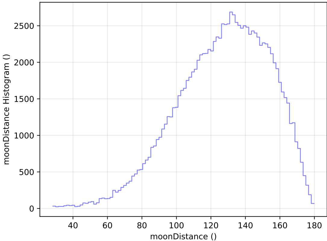
baseline_v3.0_10yrs All sky u band: moonDistance Histogram
