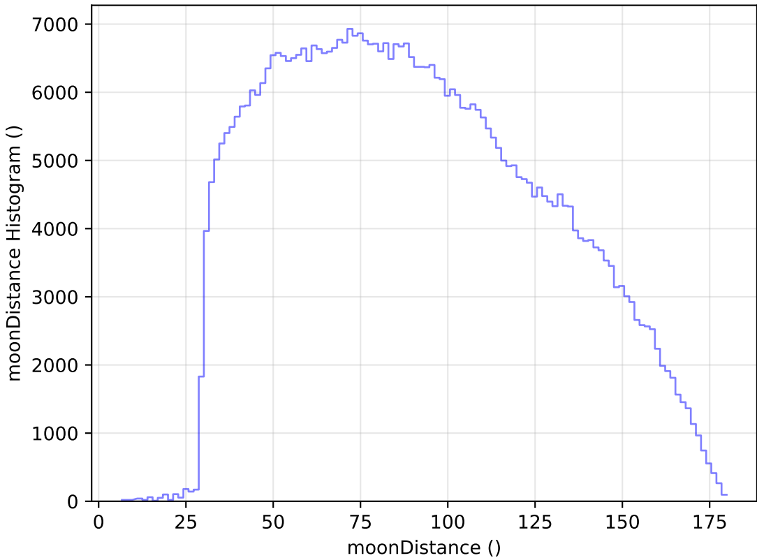
baseline_v3.0_10yrs All sky i band: moonDistance Histogram
