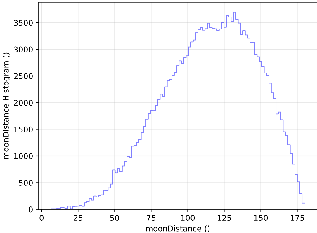
baseline_v3.0_10yrs All sky g band: moonDistance Histogram
