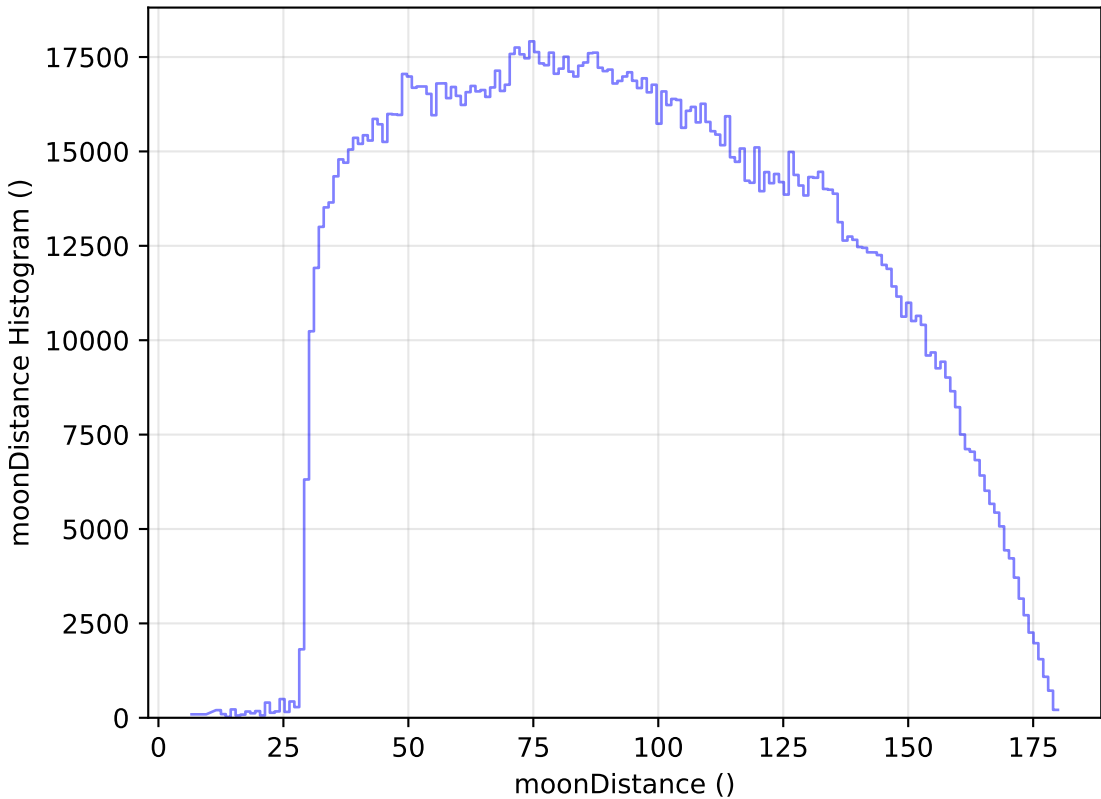
baseline_v3.0_10yrs All sky all bands: moonDistance Histogram
