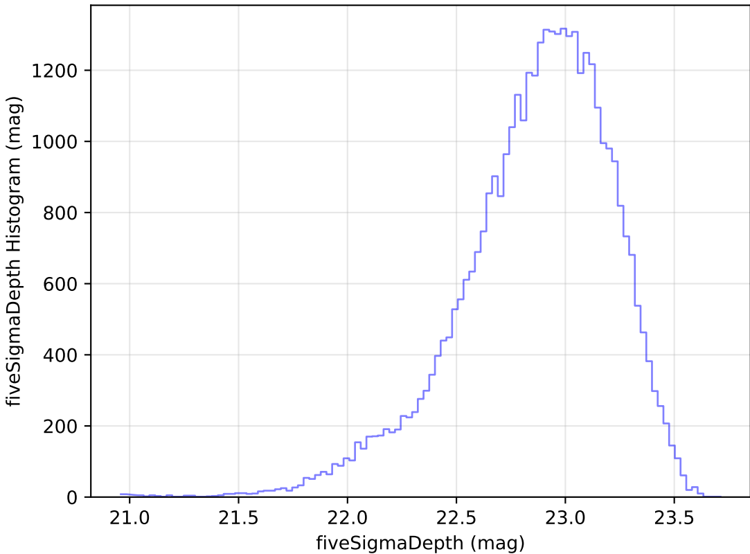
baseline_v3.0_10yrs Yr 1 z band: fiveSigmaDepth Histogram
