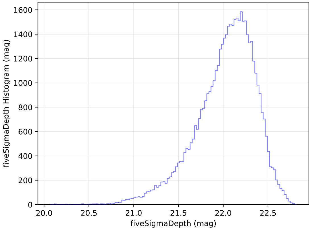
baseline_v3.0_10yrs Yr 1 y band: fiveSigmaDepth Histogram
