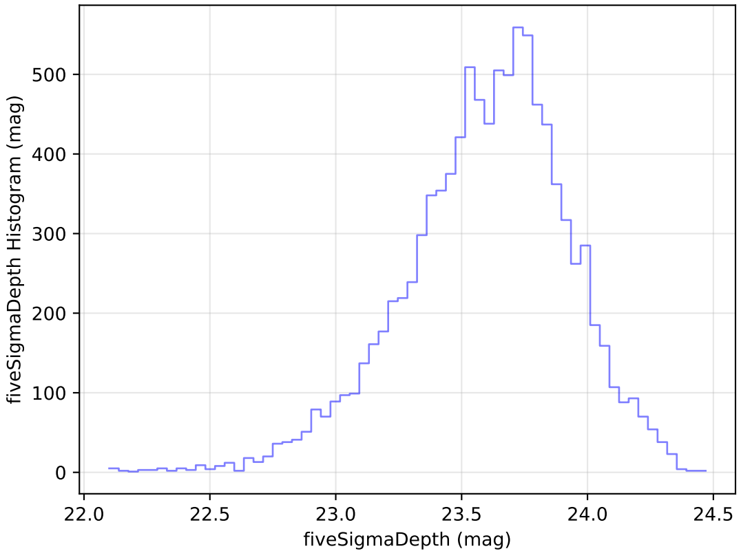
baseline_v3.0_10yrs Yr 1 u band: fiveSigmaDepth Histogram
