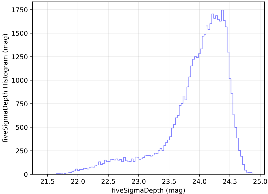
baseline_v3.0_10yrs Yr 1 r band: fiveSigmaDepth Histogram
