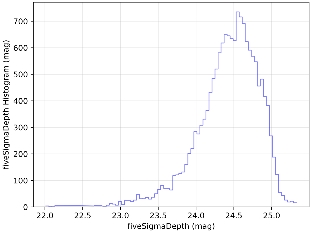
baseline_v3.0_10yrs Yr 1 g band: fiveSigmaDepth Histogram
