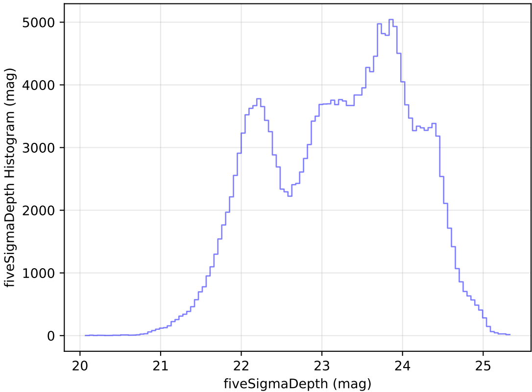
baseline_v3.0_10yrs Yr 1 all bands: fiveSigmaDepth Histogram
