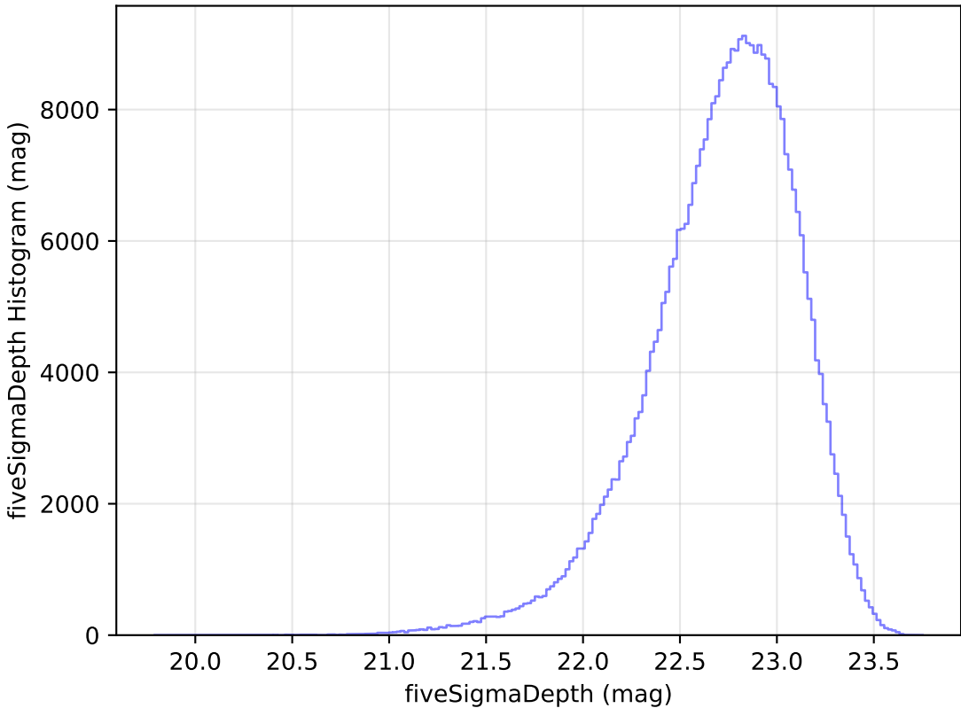
baseline_v3.0_10yrs WFD z band: fiveSigmaDepth Histogram
