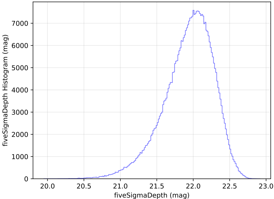
baseline_v3.0_10yrs WFD y band: fiveSigmaDepth Histogram
