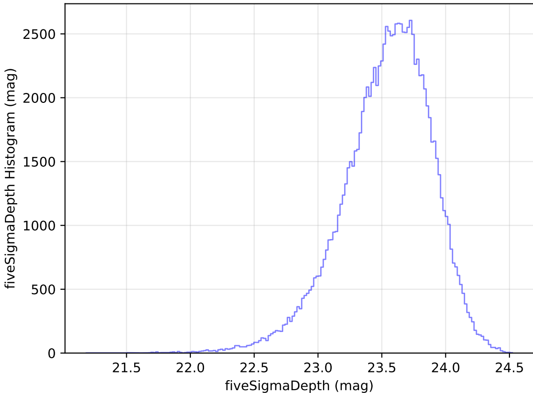
baseline_v3.0_10yrs WFD u band: fiveSigmaDepth Histogram
