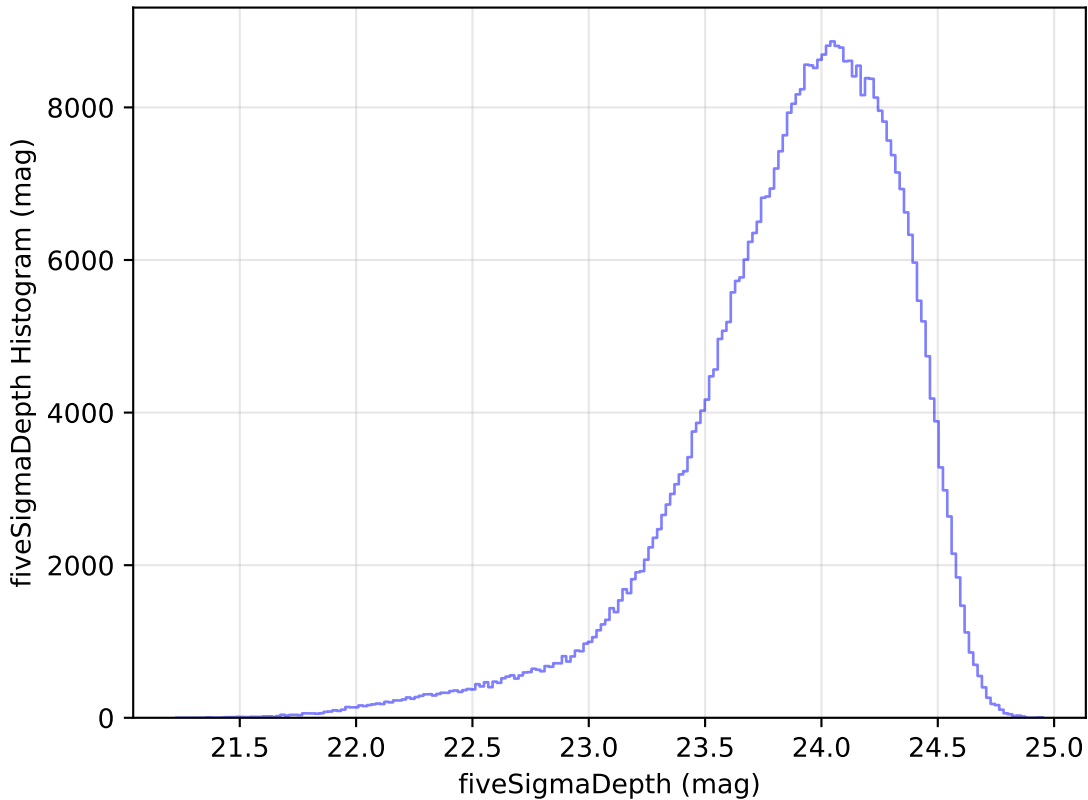
baseline_v3.0_10yrs WFD r band: fiveSigmaDepth Histogram
