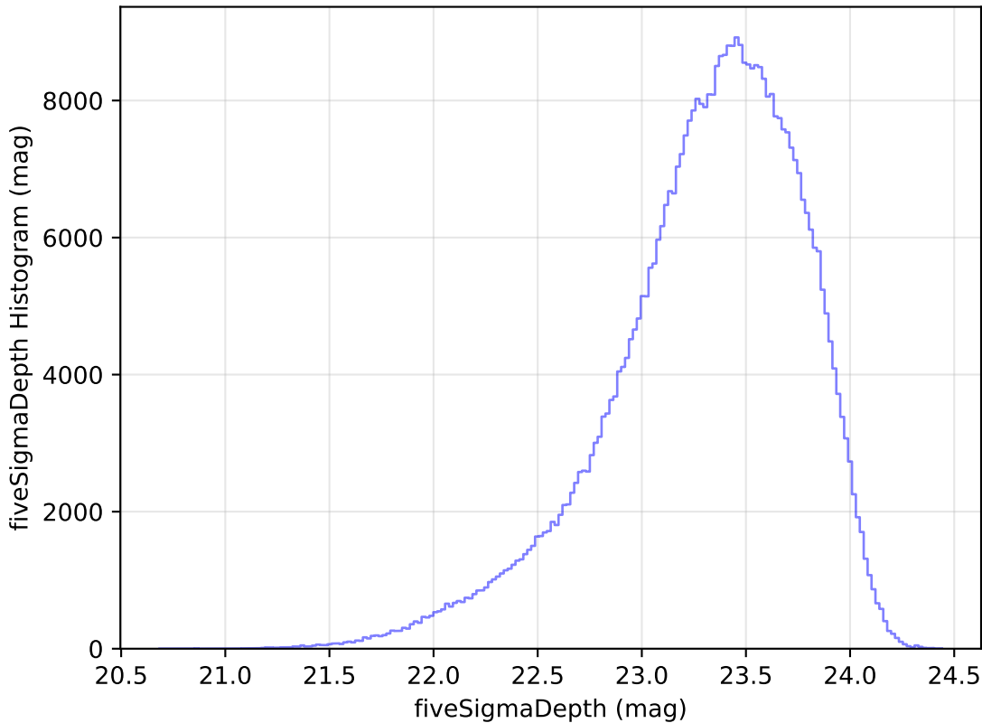
baseline_v3.0_10yrs WFD i band: fiveSigmaDepth Histogram
