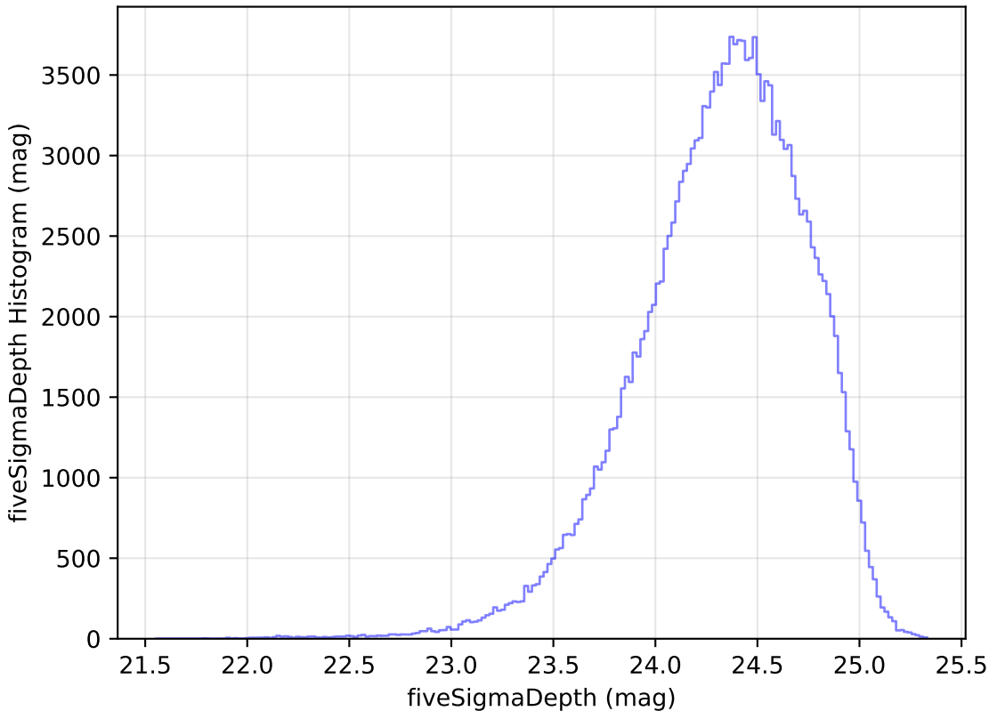
baseline_v3.0_10yrs WFD g band: fiveSigmaDepth Histogram
