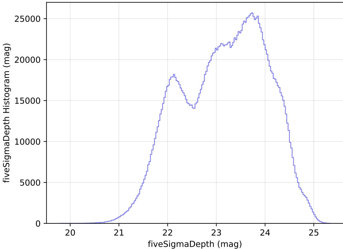
baseline_v3.0_10yrs WFD all bands: fiveSigmaDepth Histogram
