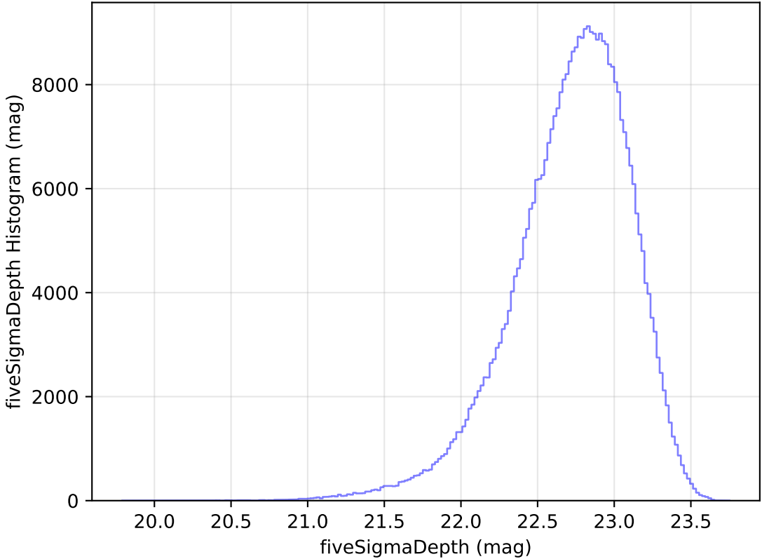
baseline_v3.0_10yrs All sky z band: fiveSigmaDepth Histogram
