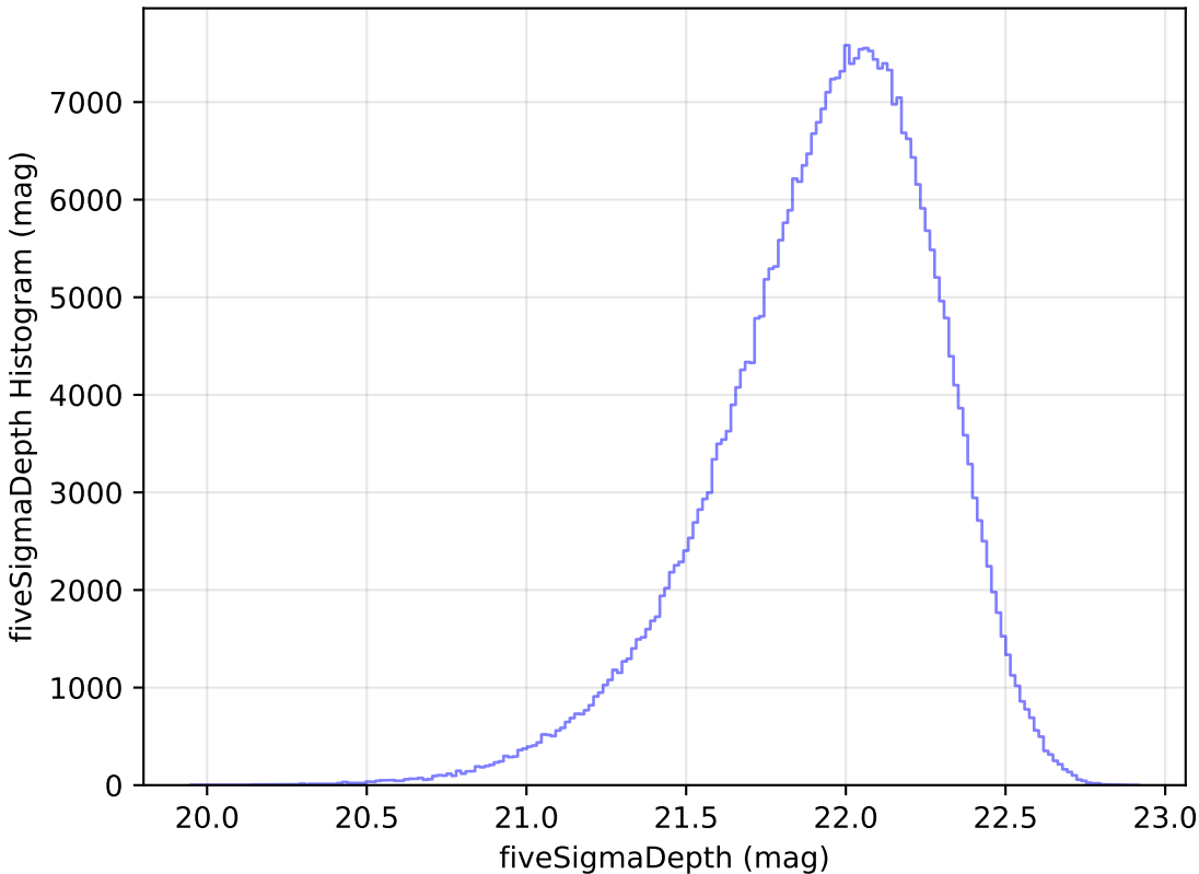
baseline_v3.0_10yrs All sky y band: fiveSigmaDepth Histogram
