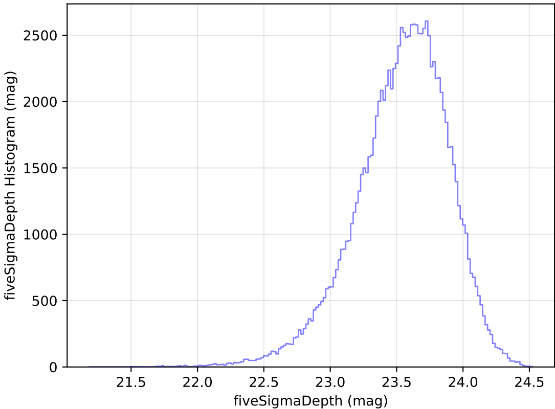
baseline_v3.0_10yrs All sky u band: fiveSigmaDepth Histogram
