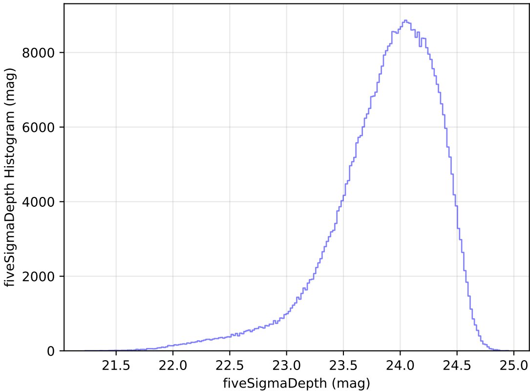
baseline_v3.0_10yrs All sky r band: fiveSigmaDepth Histogram
