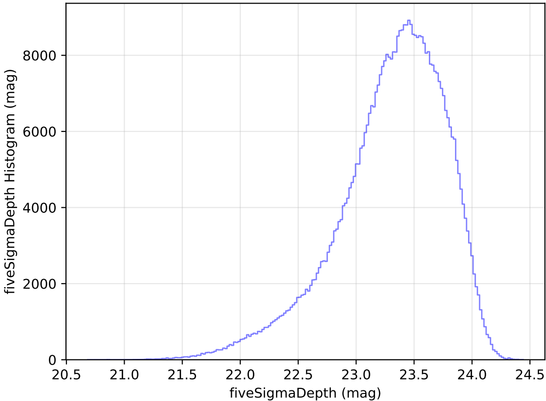
baseline_v3.0_10yrs All sky i band: fiveSigmaDepth Histogram
