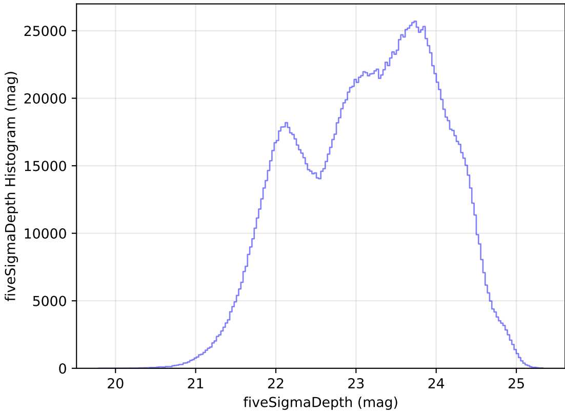
baseline_v3.0_10yrs All sky all bands: fiveSigmaDepth Histogram
