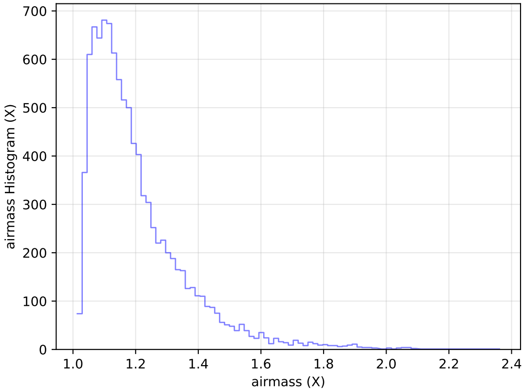
baseline_v3.0_10yrs Yr 1 u band: airmass Histogram
