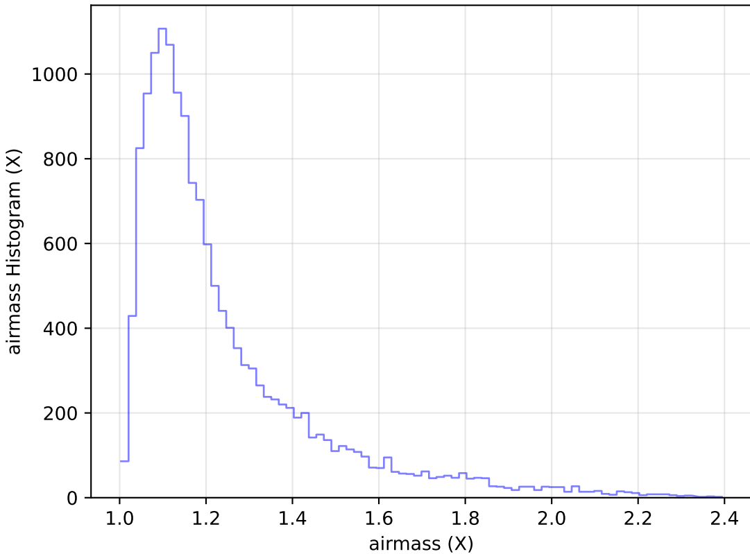
baseline_v3.0_10yrs Yr 1 g band: airmass Histogram
