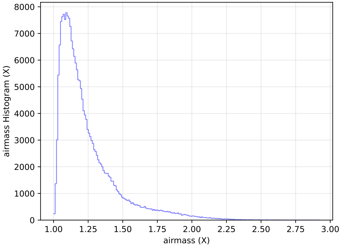
baseline_v3.0_10yrs Yr 1 all bands: airmass Histogram
