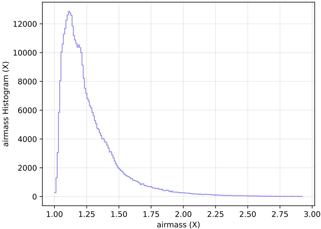
baseline_v3.0_10yrs WFD y band: airmass Histogram
