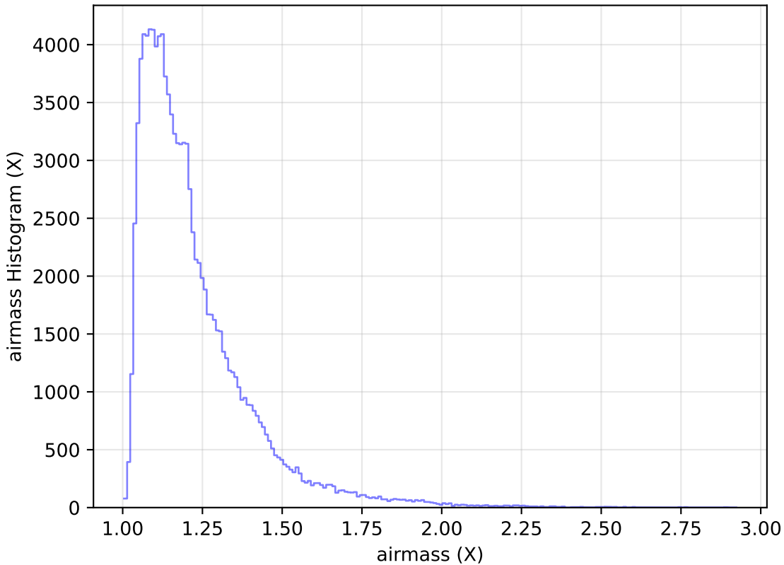
baseline_v3.0_10yrs WFD u band: airmass Histogram
