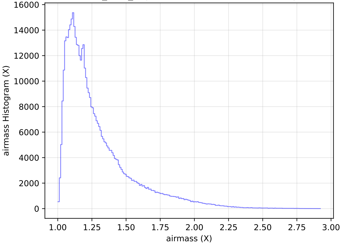
baseline_v3.0_10yrs WFD i band: airmass Histogram
