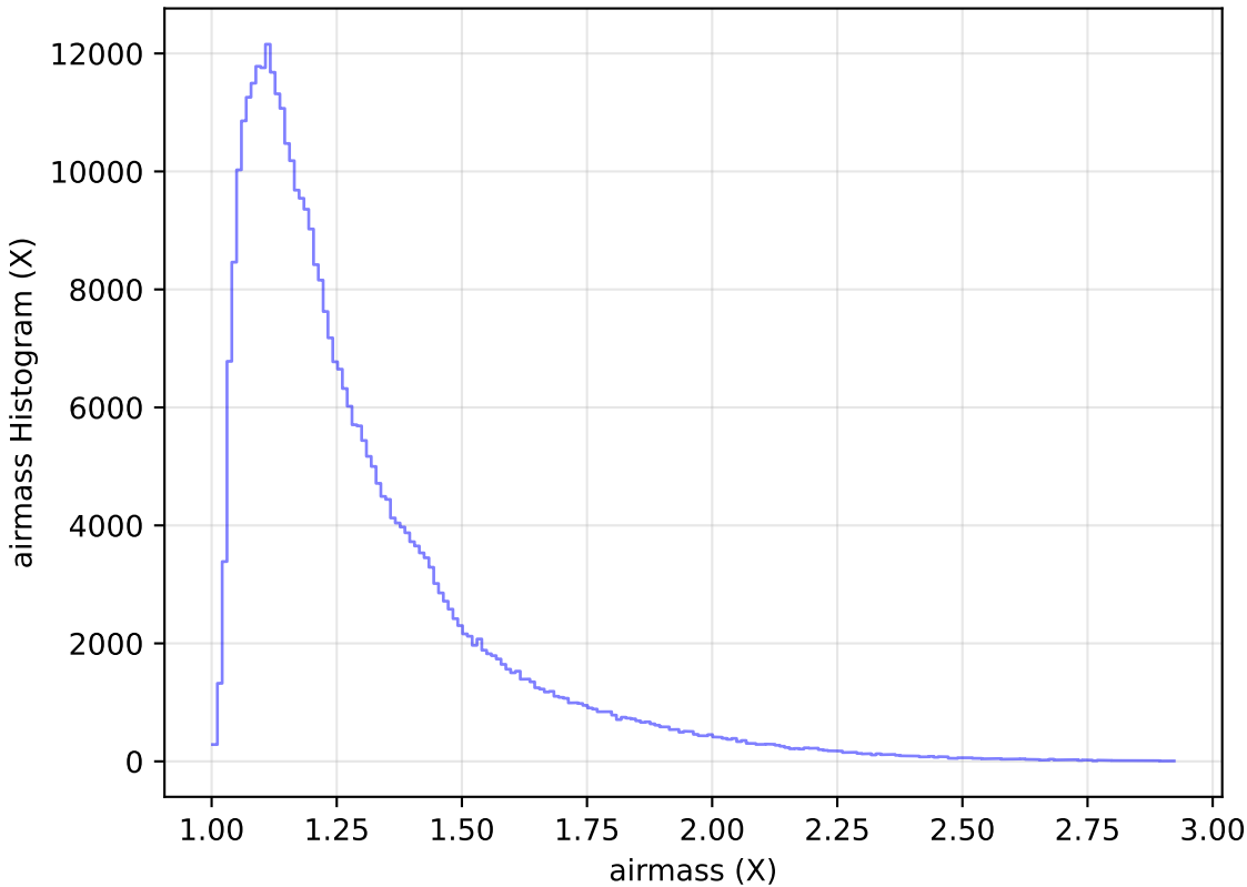
baseline_v3.0_10yrs All sky z band: airmass Histogram
