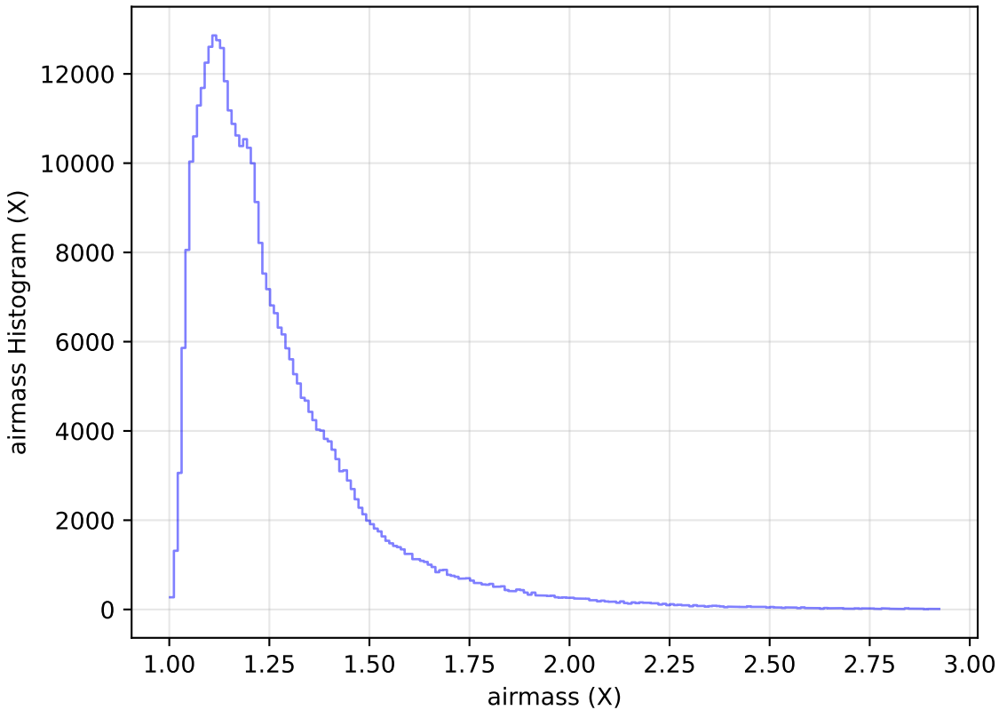
baseline_v3.0_10yrs All sky y band: airmass Histogram
