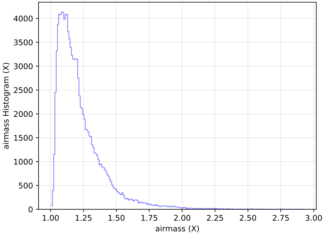
baseline_v3.0_10yrs All sky u band: airmass Histogram
