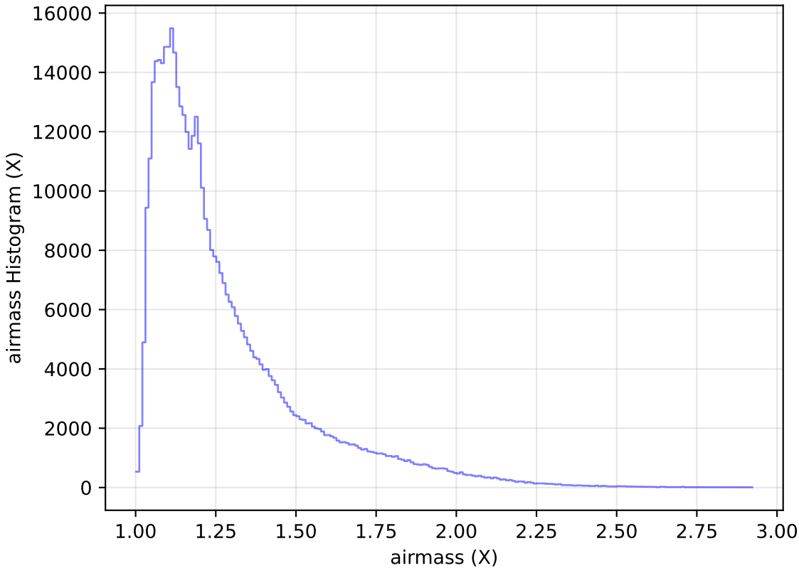
baseline_v3.0_10yrs All sky r band: airmass Histogram
