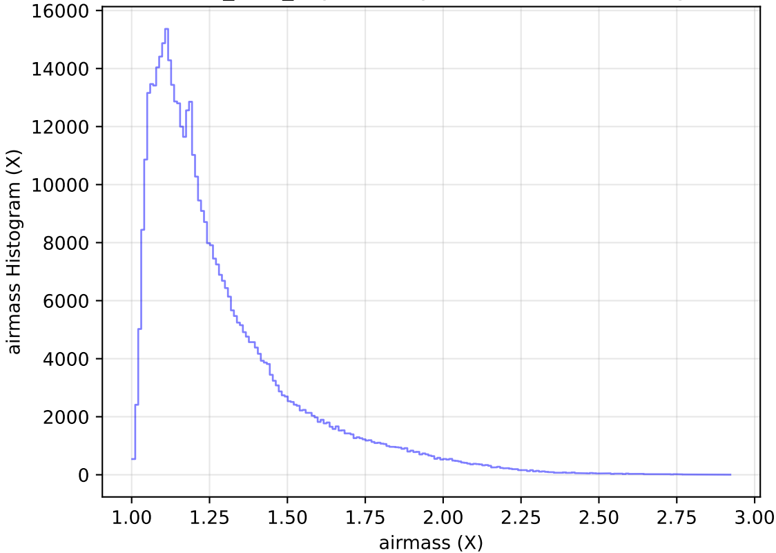
baseline_v3.0_10yrs All sky i band: airmass Histogram
