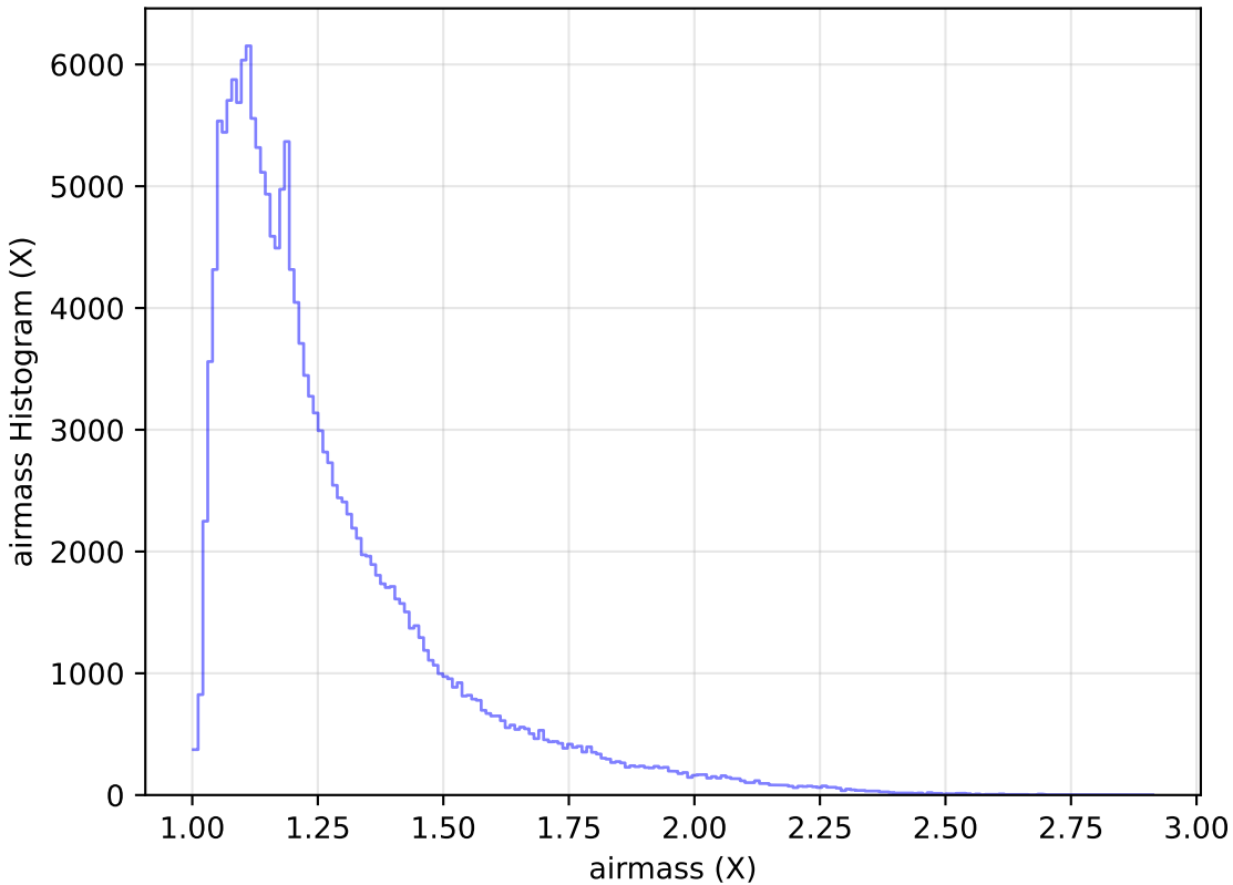
baseline_v3.0_10yrs All sky g band: airmass Histogram
