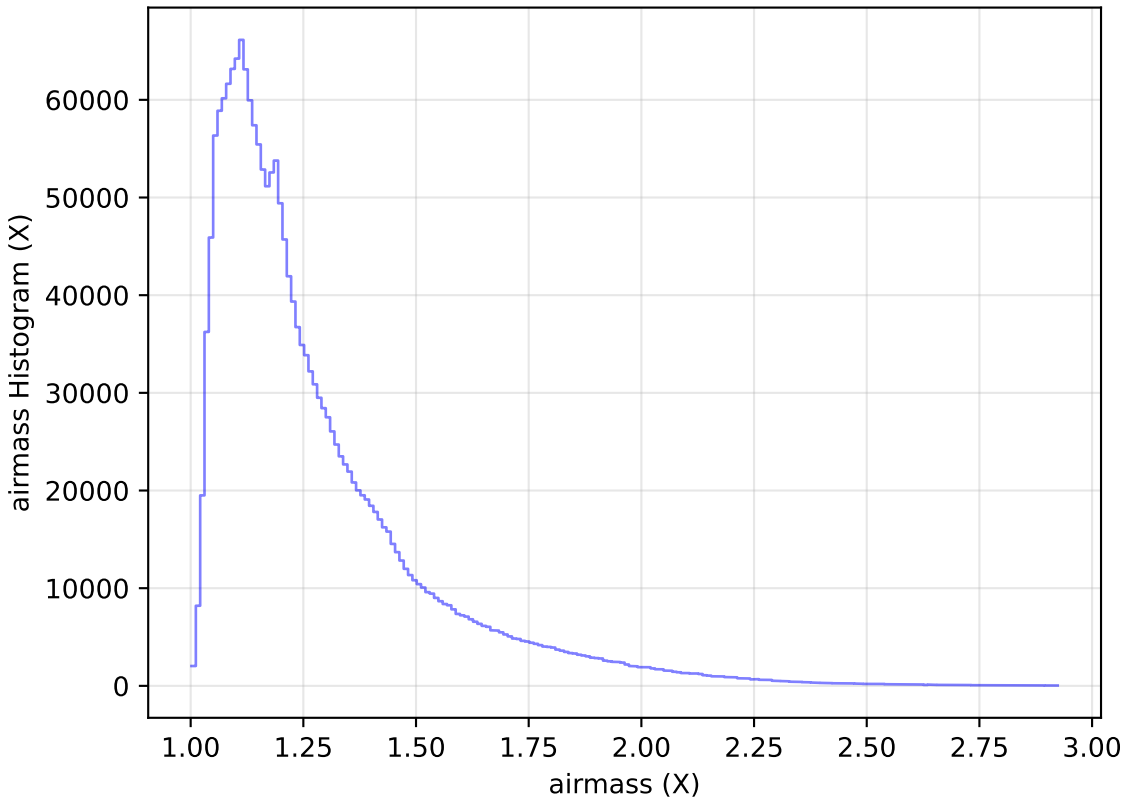
baseline_v3.0_10yrs All sky all bands: airmass Histogram
