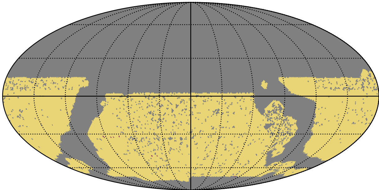
baseline_v3.0_10yrs WFD: RapidRevisits
