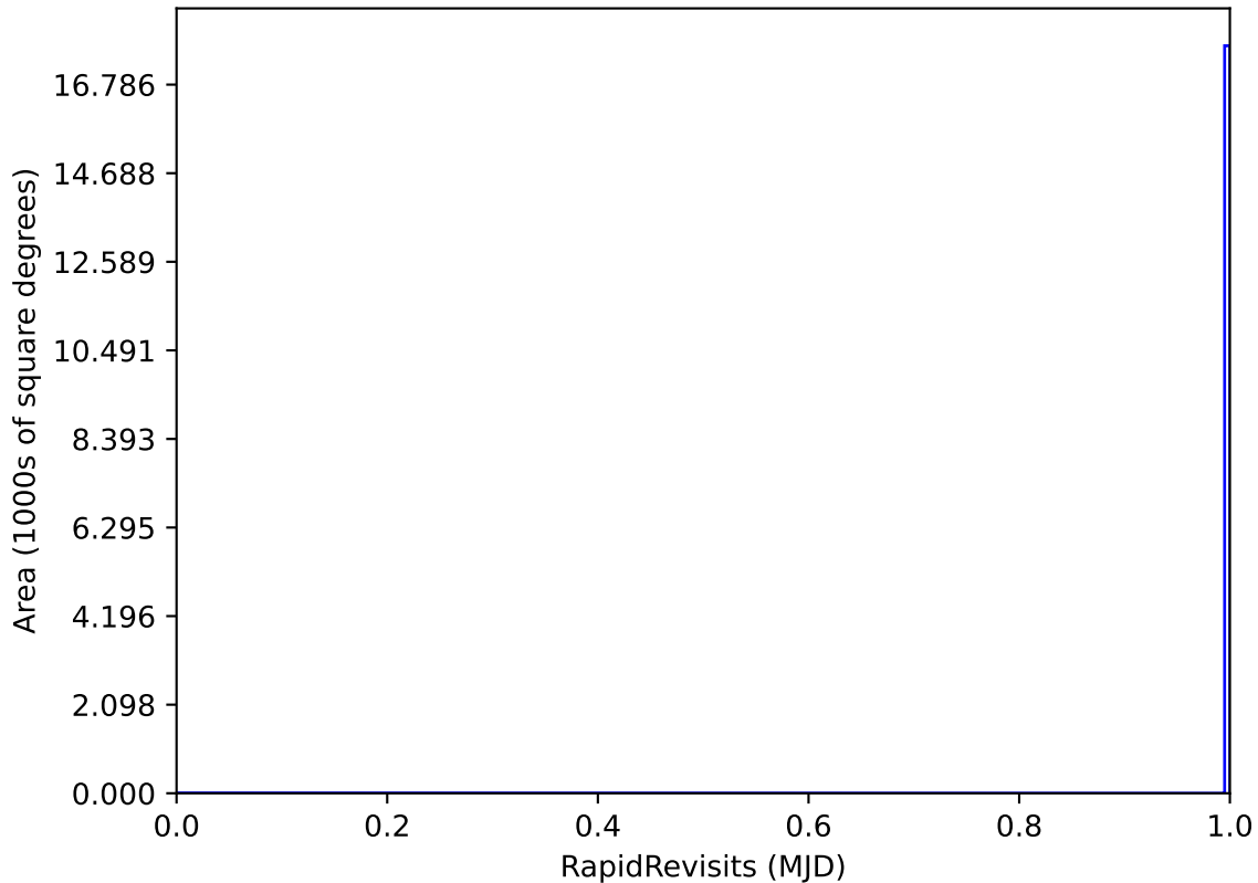
baseline_v3.0_10yrs WFD: RapidRevisits
