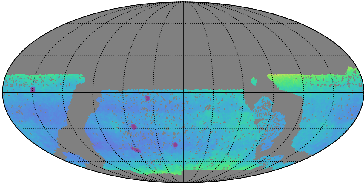
baseline_v3.0_10yrs WFD: Proper Motion Uncert @ 24.0
