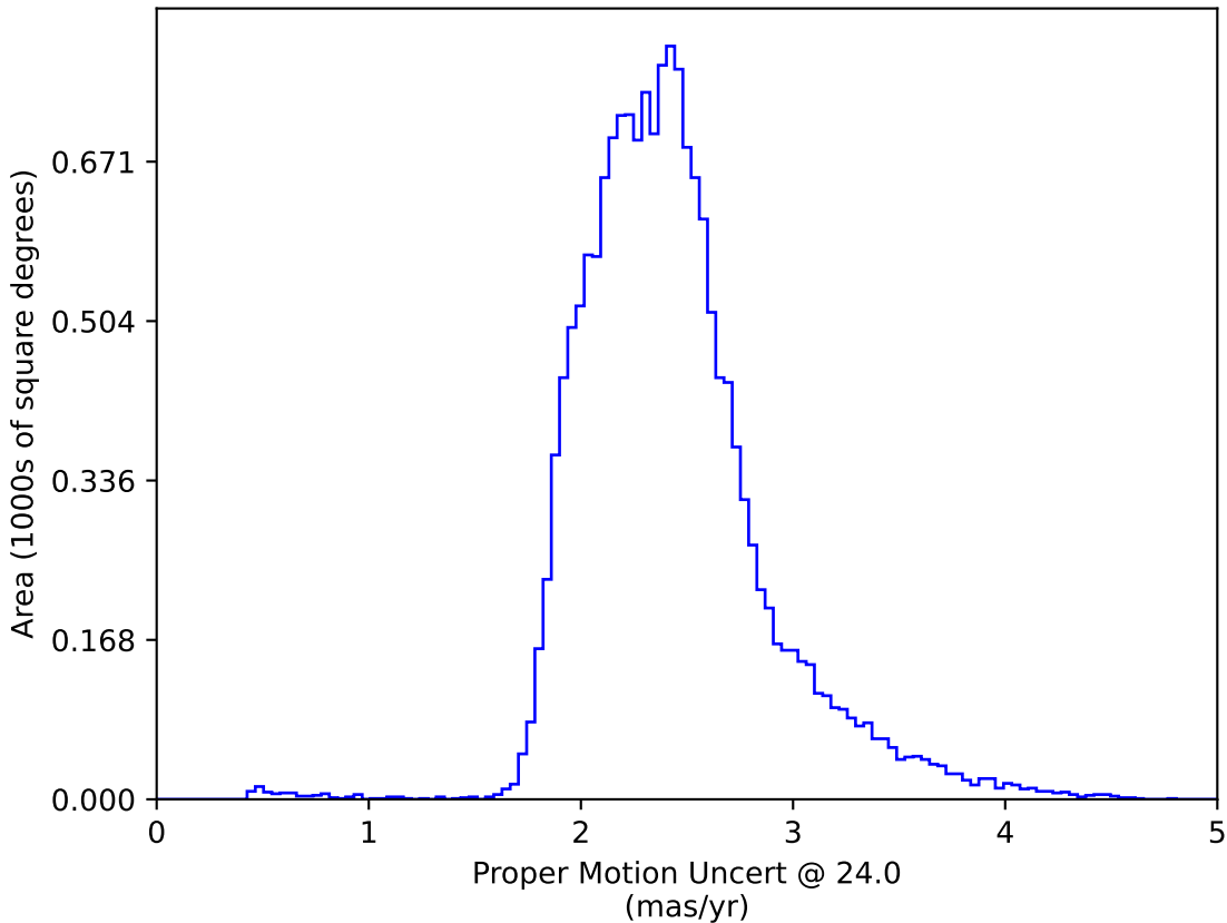
baseline_v3.0_10yrs WFD: Proper Motion Uncert @ 24.0
