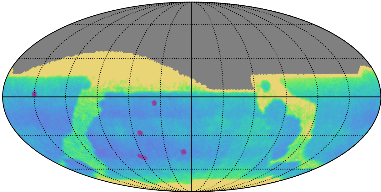
baseline_v3.0_10yrs All sky: Proper Motion Uncert @ 24.0
