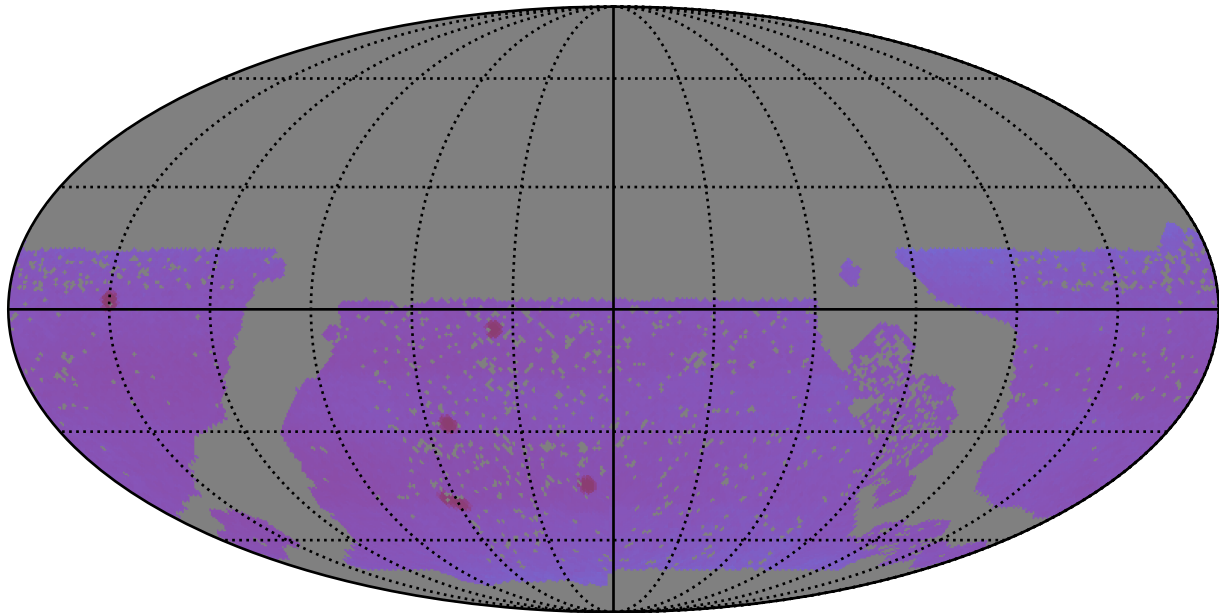
baseline_v3.0_10yrs WFD: Proper Motion Uncert @ 20.5
