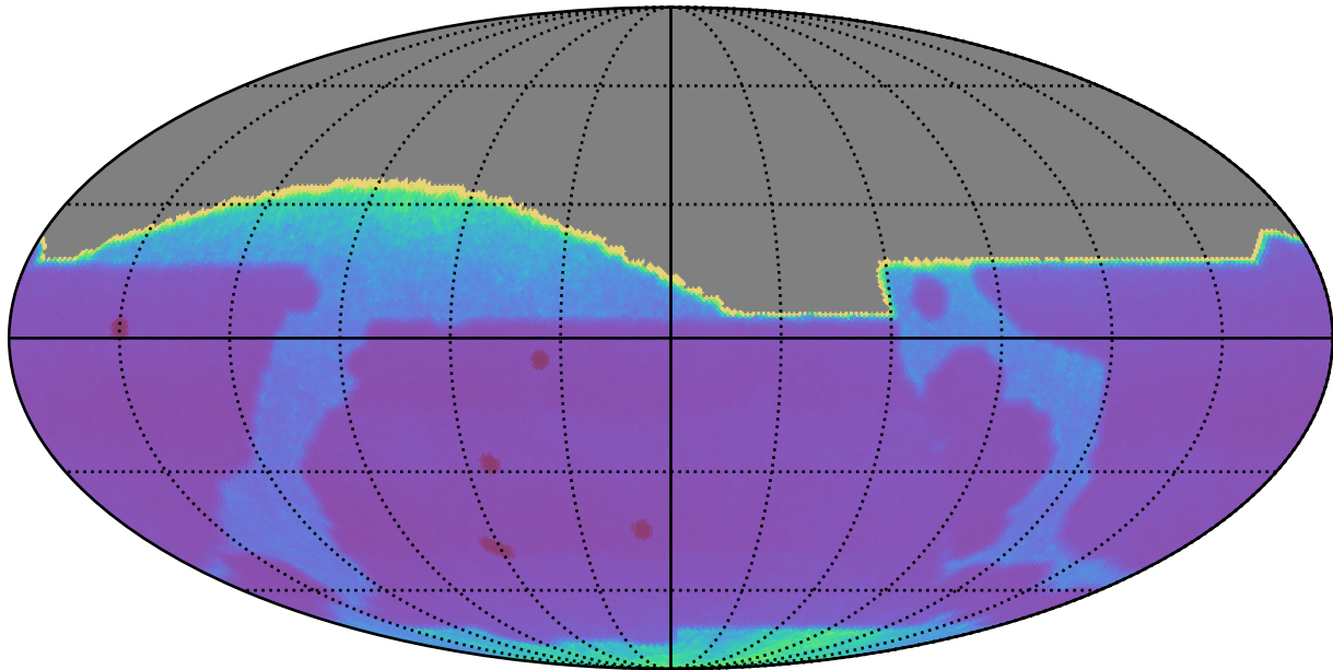
baseline_v3.0_10yrs All sky: Proper Motion Uncert @ 20.5
