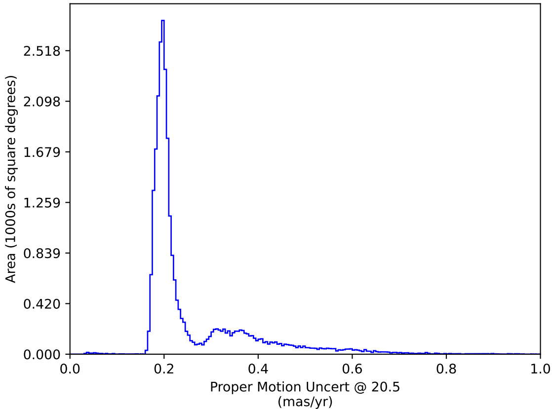
baseline_v3.0_10yrs All sky: Proper Motion Uncert @ 20.5
