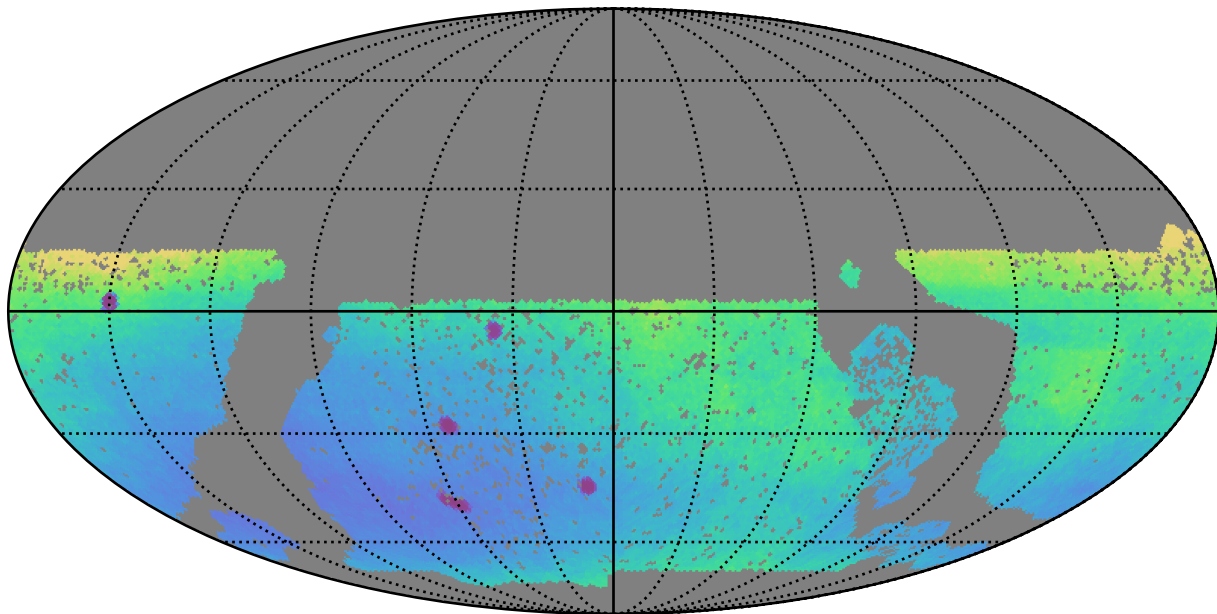
baseline_v3.0_10yrs WFD: Parallax Uncert @ 24.0
